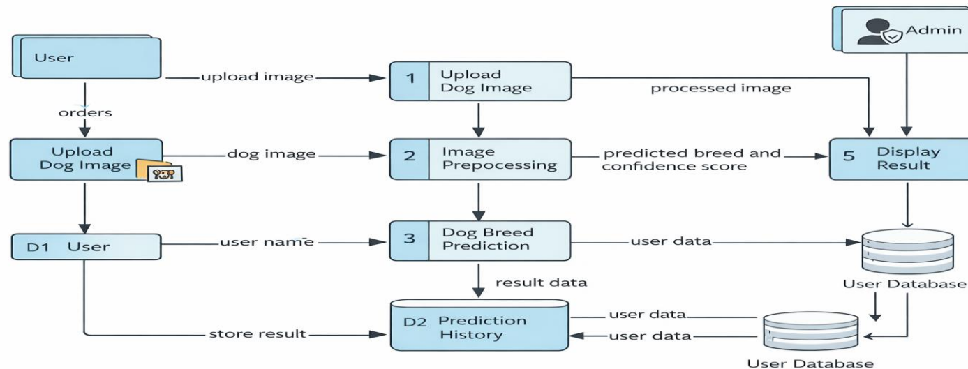
Dog Breed Identification System Using Transfer Learning - DFD Level 0
